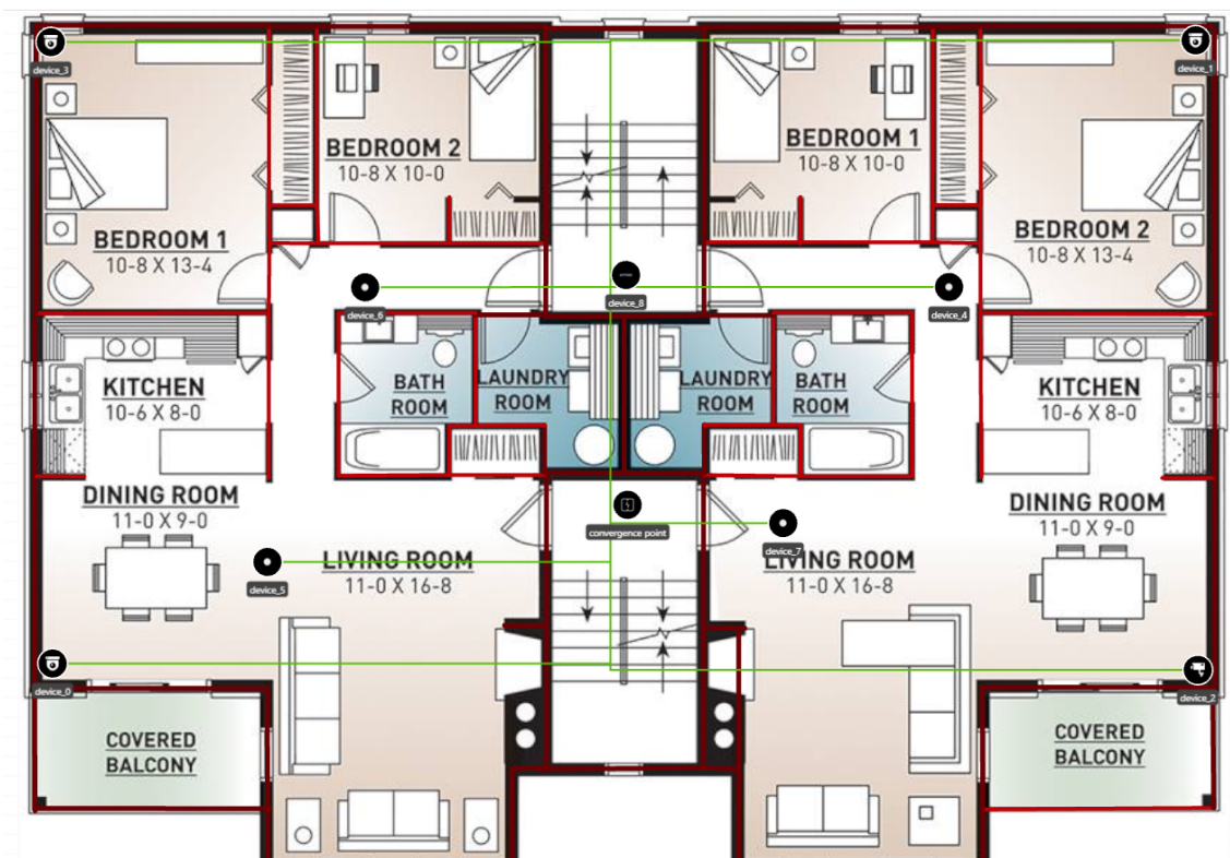
Figure 2-31 Cabling Design
