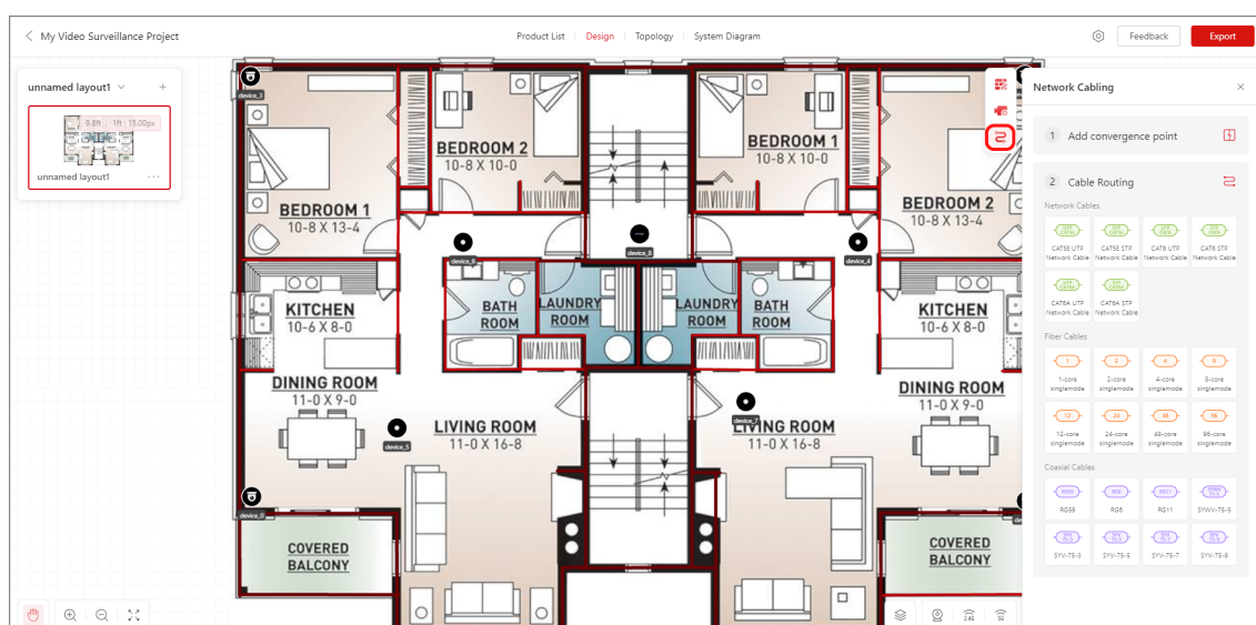
Figure 2-28 Cabling Design
